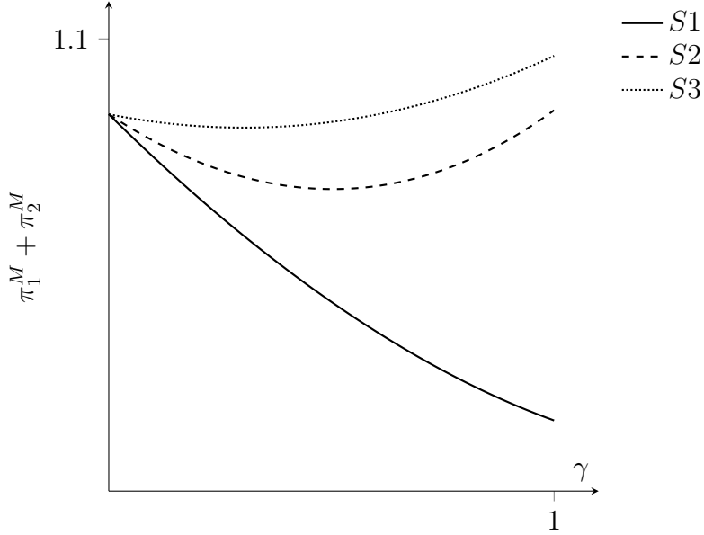
Figure 5: Sum of profits of firms 1 and 2 as a function of \gamma in our three scenarios.
