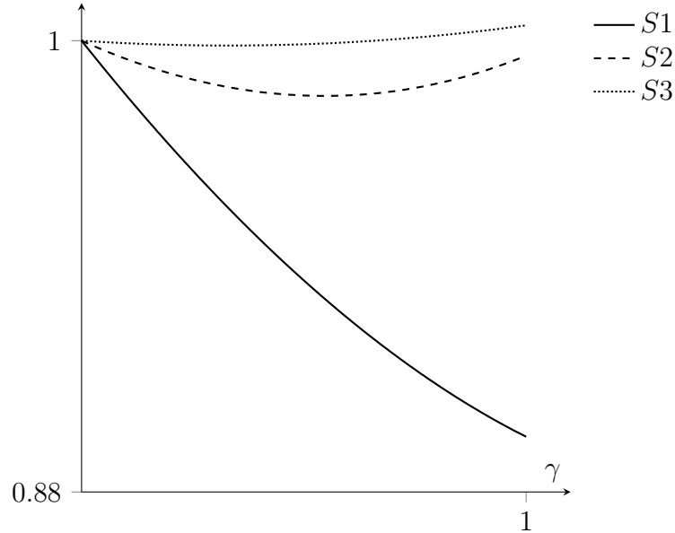
Figure 4: Costs borne by consumers as a function of \gamma in our three scenarios.
