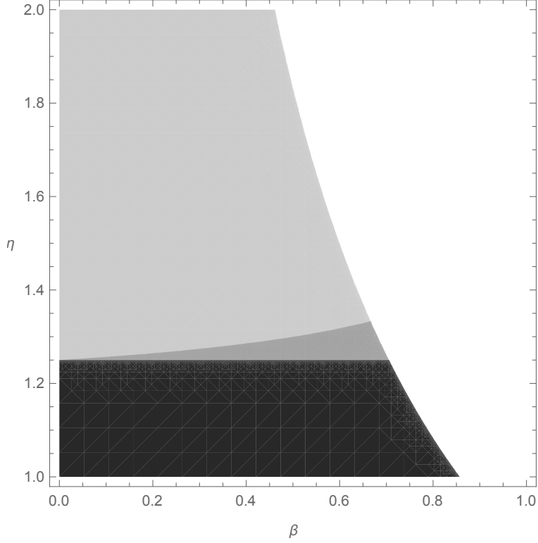
Figure 1: Combinations of \beta and \eta analyzed in the body (light-grey area) or in Appendix D (dark-grey and black areas) of the paper
