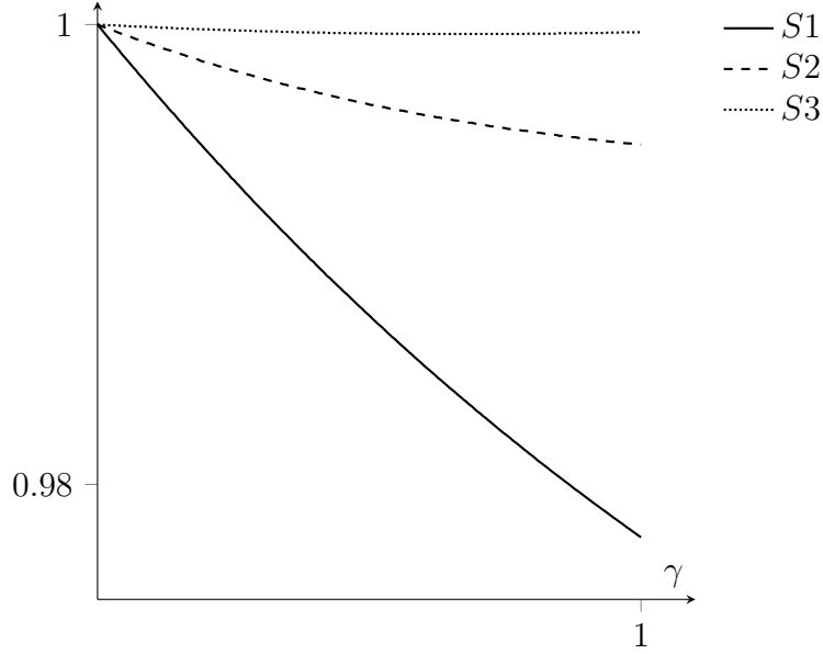
Figure 6: Social costs as a function of \gamma in our three scenarios.
