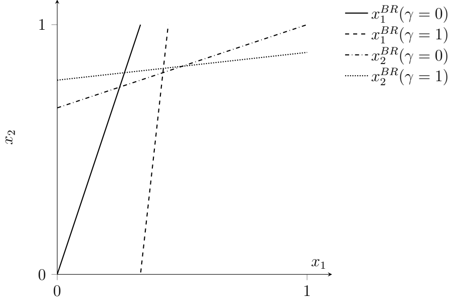
Figure 2: Firms' product safety best-response functions under no compensation ( \gamma = 0 ) and full compensation ( \gamma = 1 ) for \underline{h} = 1 , a = 5/2 , and \beta = 1/2 .
