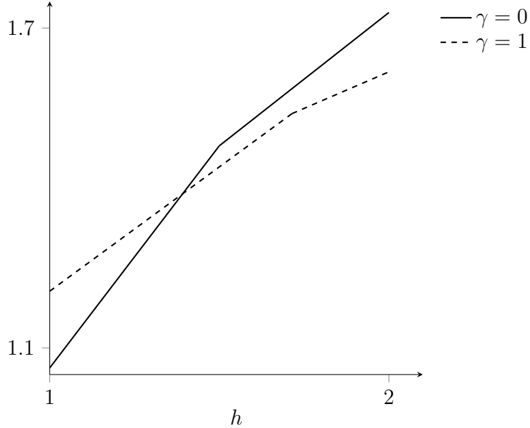
Figure 3: Costs of consumers under no compensation ( \gamma = 0 ) and full compensation ( \gamma = 1 ) for \underline{h} = 1 , a = 9/2 , and \beta = 1/3 .
